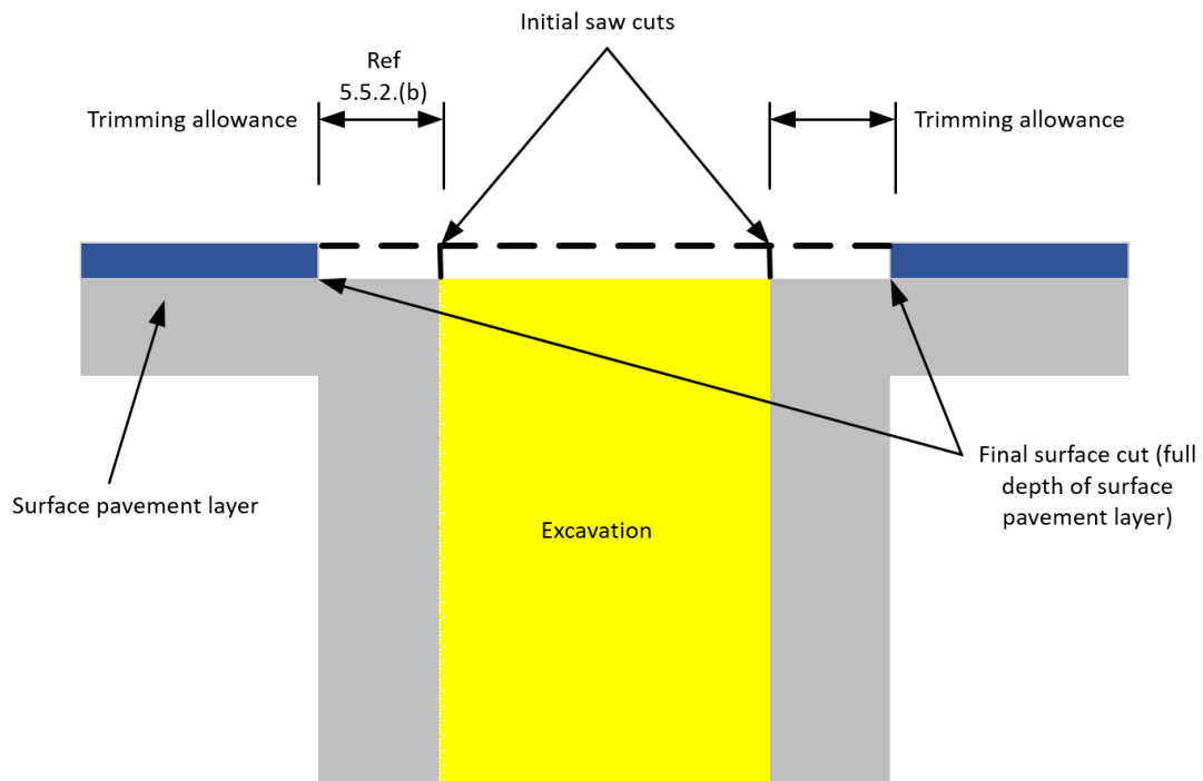
Figure 5-3 Procedures for Working in Road and Motorway Corridors -3: Standard trimming for Trench cuts
