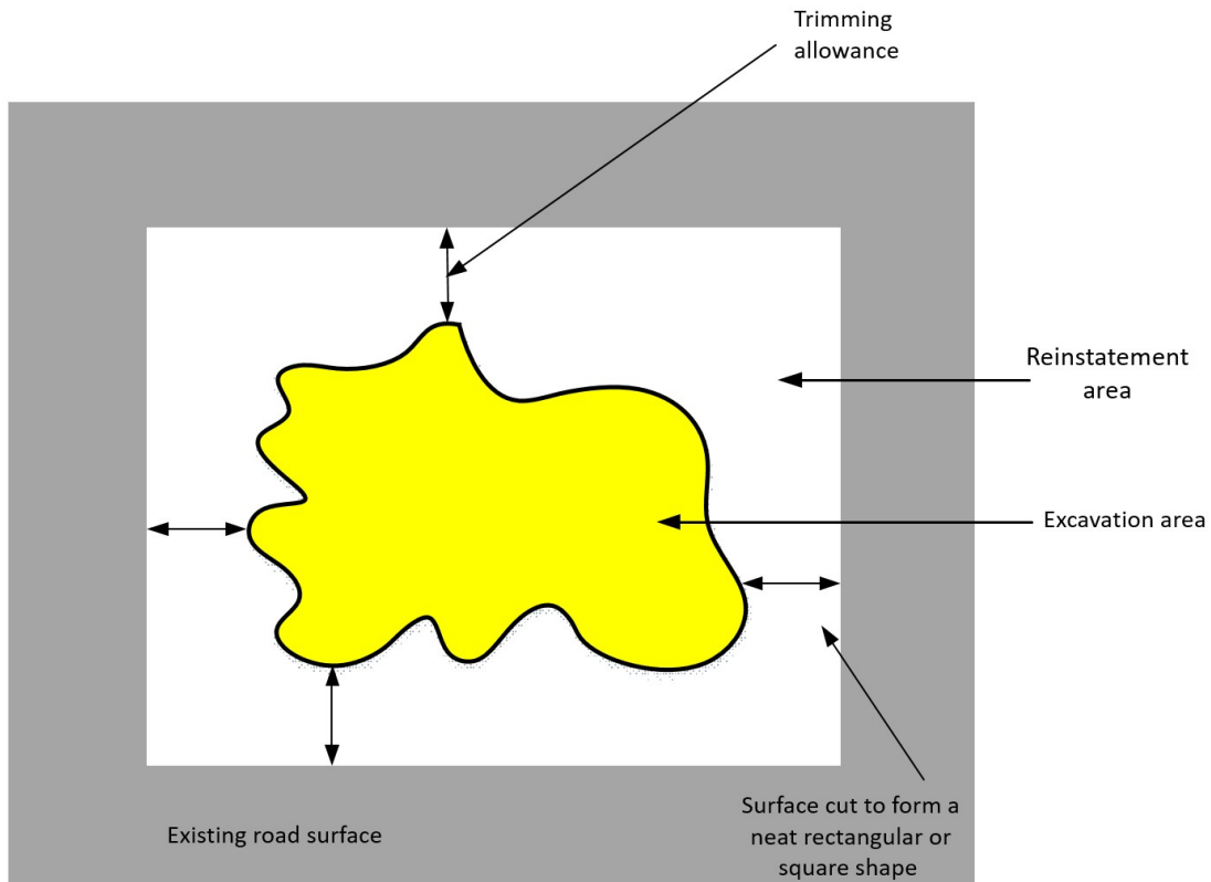
Figure 5-6 Procedures for Working in Road and Motorway Corridors -6: Finishing of irregular shaped excavations
