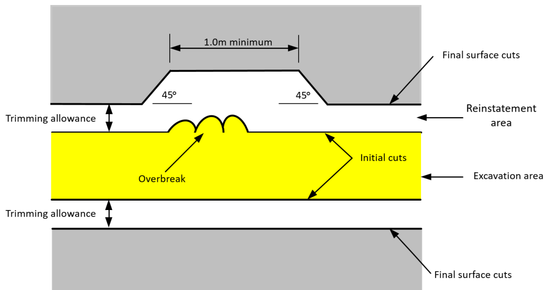
Figure 5-3 Procedures for Working in Road and Motorway Corridors -3: Standard trimming for Trench cuts
